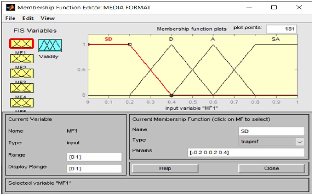
Figure 6. Fuzzy input for media format
