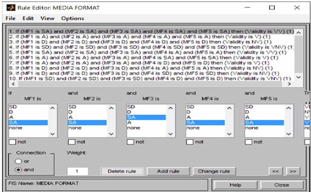
Figure 8. Fuzzy inference rule for media format
